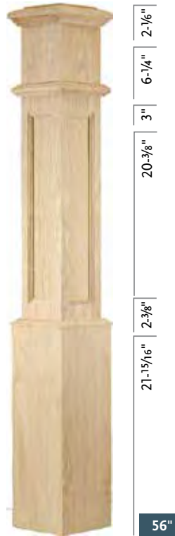
C-4891-FP Flat Panel Base Width 7-1/2" RO, POP, PRM
