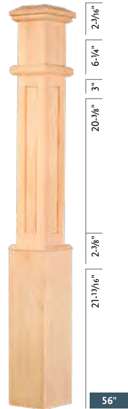
C-4790 Mission Base Width 6-1/4" RO, POP, PRM
