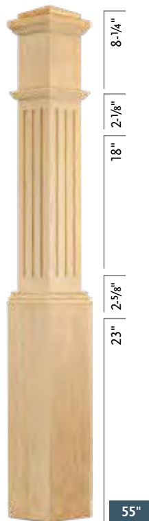
C-4091-F Fluted Base Width 6-1/4" RO, POP, PRM, HM
