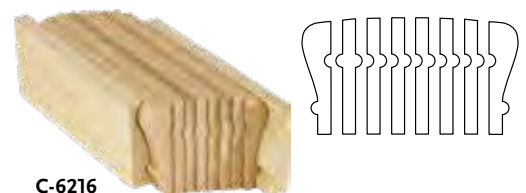
C-6216 Bending Rail 2-5/8" x 2-3/8" Avail: 12', 16', 18', 20'
