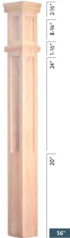
C-4092 Craftsman Base Width 5" RO, PRM, WO
