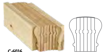
C-6016 Bending Rail 2-3/4" x 2-3/8"
