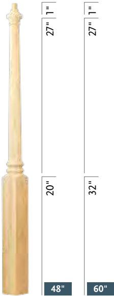
Base Width 3" RO
