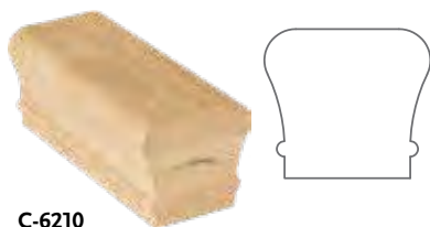
C-6210 Non-Plowed 2-5/8" x 2-3/8" Avail: FJ, SC, ENG
