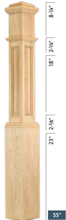
C-4091-RP Raised Panel Base Width 6-1/4" RO, POP, PRM, HM, WO
